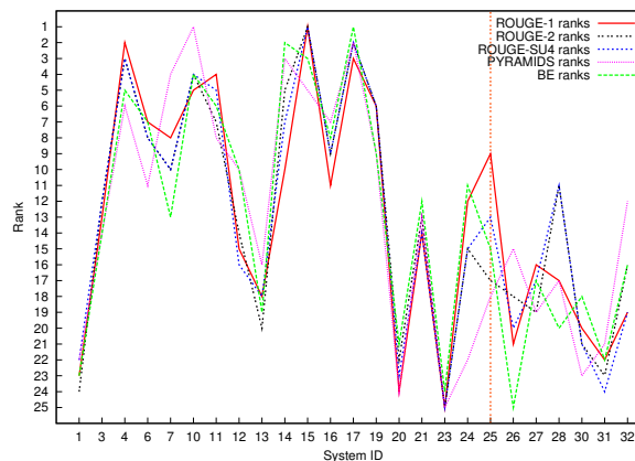
Figure 3: System ranks based on ROUGE and Pyramid scores (systems participating in Pyramid evaluation only)
